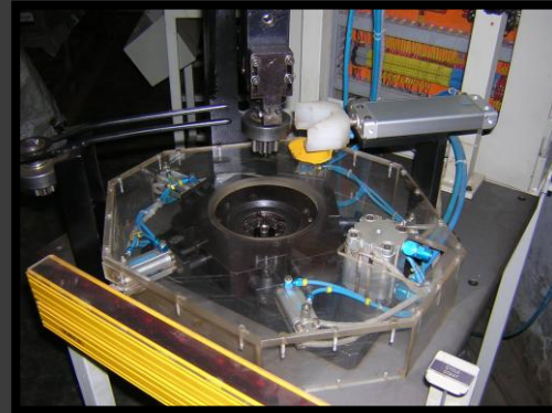
Roller and Spring Assembly for Self Starter - Drive
